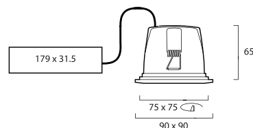
Insaver 75 LED Square
