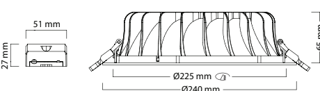
Syl-Lighter LED II - Emergency Pack
