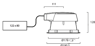
Insaver 175 LED Low Glare
