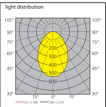
Orbito LED 4,000K
