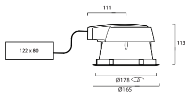
Insaver 150 LED Low Glare
