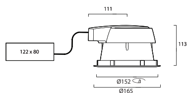
Insaver 150 LED Low Glare
