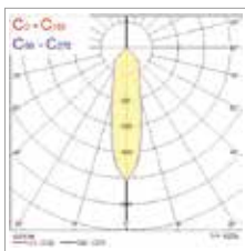
Expospot 90 Fixed HO RA80 4,000K NB White
