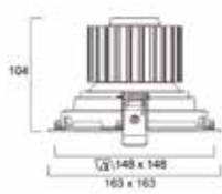
Expospot 90mm Single Square Gimbal
