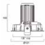
Expospot 50mm Adjustable
