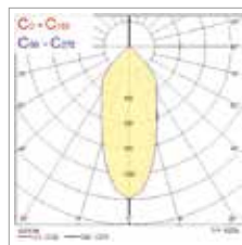
Expospot 90 Fixed HO RA80 4,000K MB White
