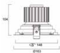
Expospot 90mm Single Round Gimbal
